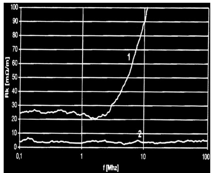
1 ... Sheet shielding 2 ... FSheet and braided shielding
